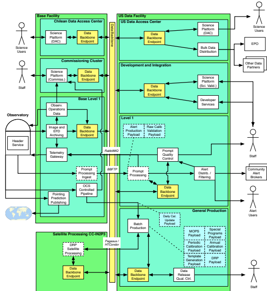
Figure 3. Rubín DM architecture diagram Lim et al. (2020)
